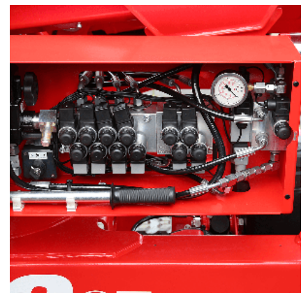
Optional available - additional hydraulic drive with electric drive
